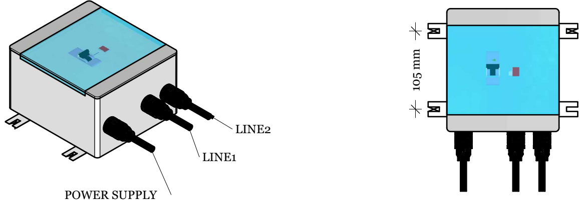
CONTROL UNIT
